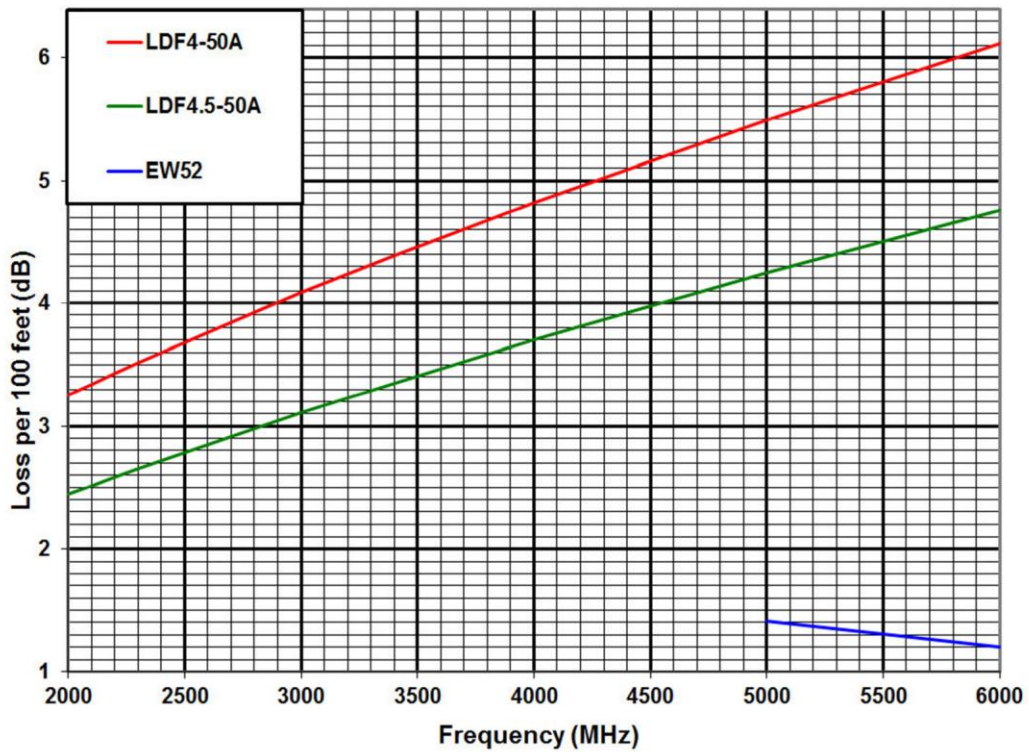
Andrew Heliax Cable and Waveguide Loss
