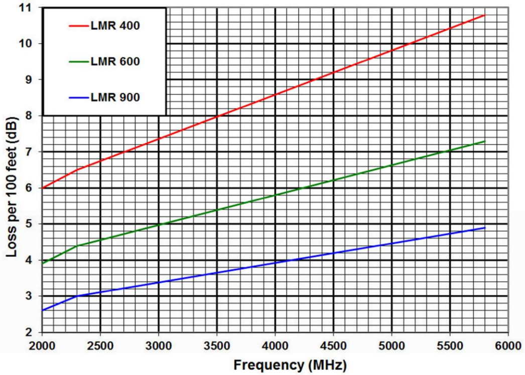
Times Microwave Cable Loss
